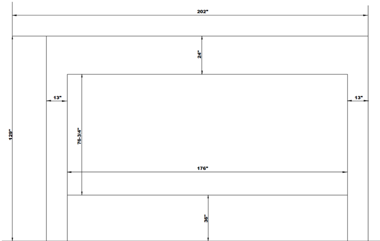
REMSEN 100 - VERTICAL MARKERBOARDS
