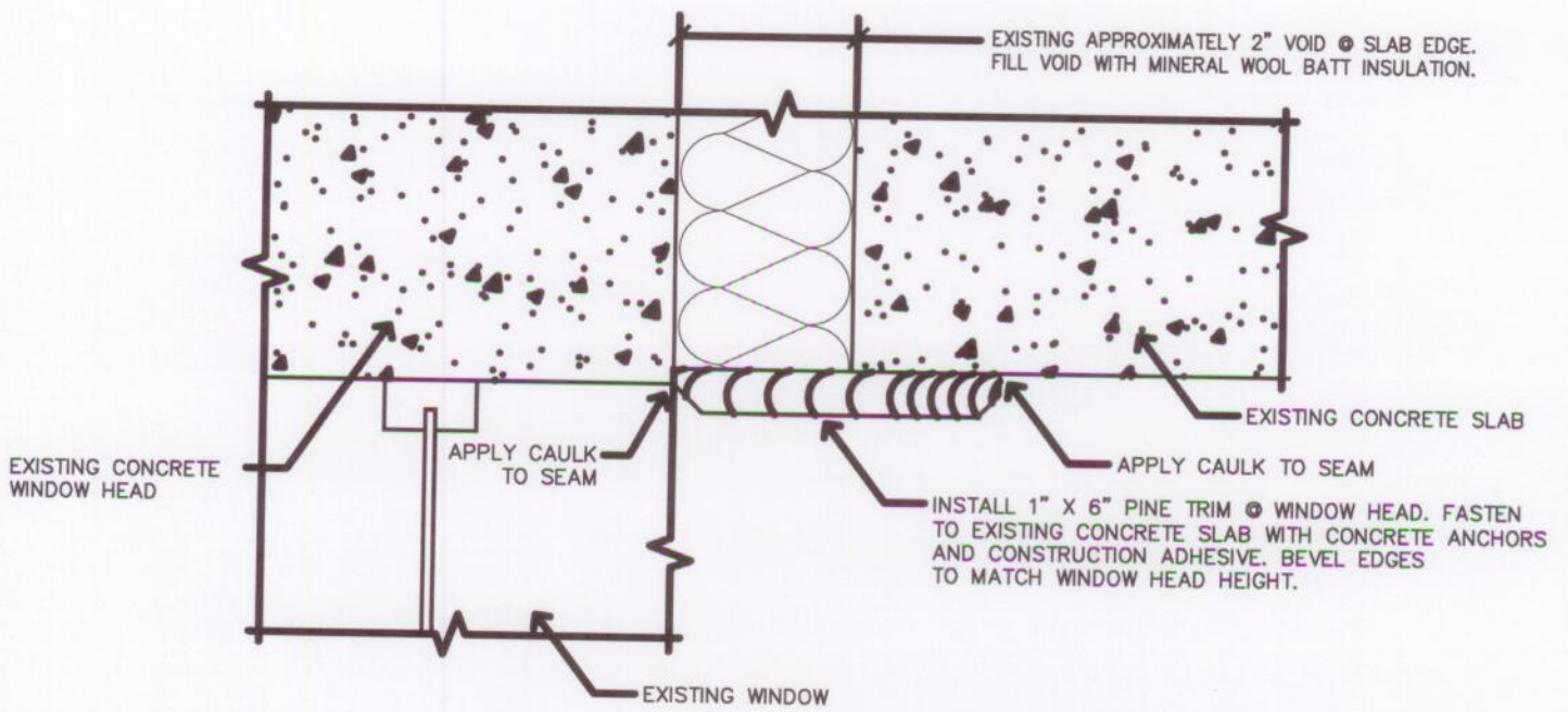
1 1" WOOD TRIM AND CAULK DETAIL SCALE: NTS
