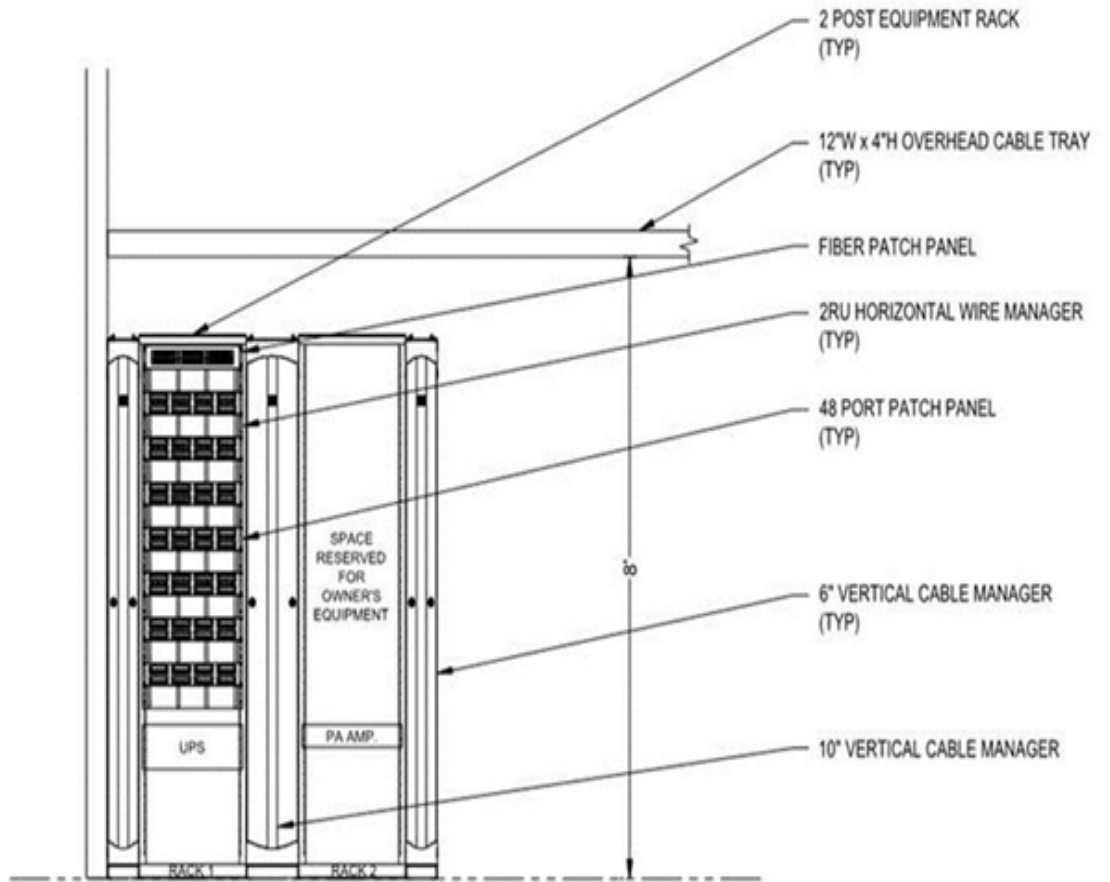
5 TELECOM ELEVATION - 2ND FLOOR IDF 1/2"=1'-0"
